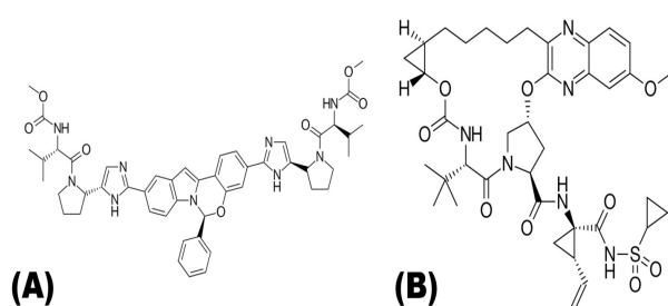
Figure 1: Chemical structures of (A) Elbasvir and (B) Grazoprevir
